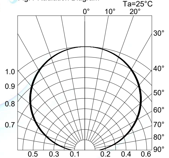
Fig.4-Radiation Diagram T_a=25^{\circ}\text{C}
