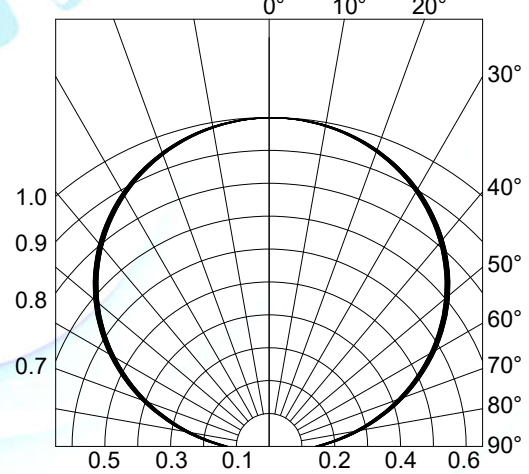
Fig.4-Radiation Diagram T_a=25^\circ\text{C}
