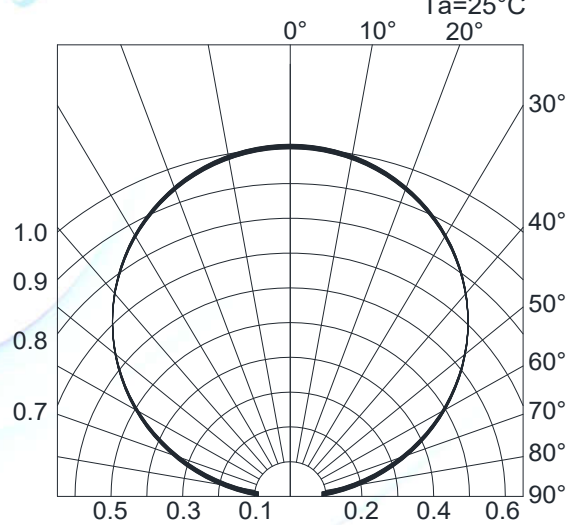
Fig.4-Radiation Diagram T_a=25^\circ\text{C}
