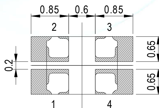
Recommended Solder Pad(2)
