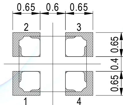
Recommended Solder Pad(2)
