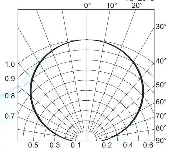
Fig.4-Radiation Diagram T_a=25^\circ\text{C}
