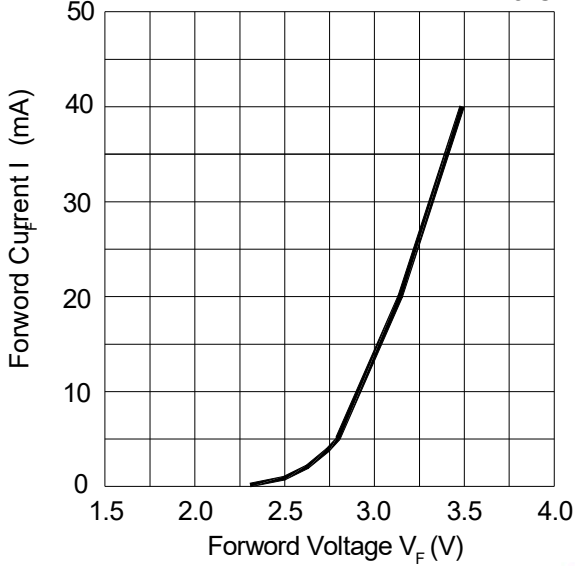
Fig.1-Forward Current(I) vs. Forward Voltage T_s=25\text{ C}
