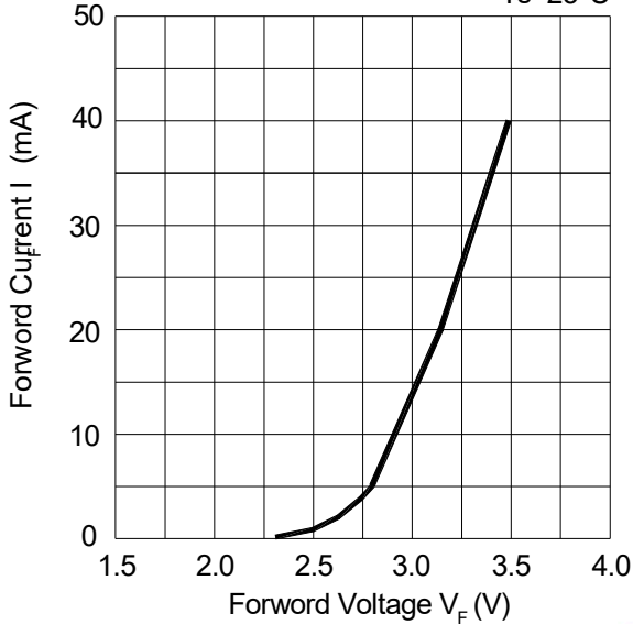
Fig.1-Forward Current(V) vs. Forward Voltage T_s=25\text{ C}
