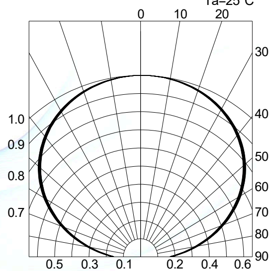
Fig.4-Radiation Diagram T_a=25\text{ C}
