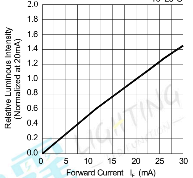
Fig.2-Relative Luminous Intensity vs. Forward Current T_s=25\text{ C}
