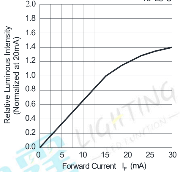
Fig.2-Relative Luminous Intensity vs. Forward Current T_s=25^{\circ}\text{C}
