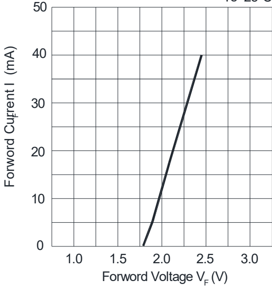
Fig.1-Forward Current(V) vs. Forward Voltage T_s=25^{\circ}\text{C}
