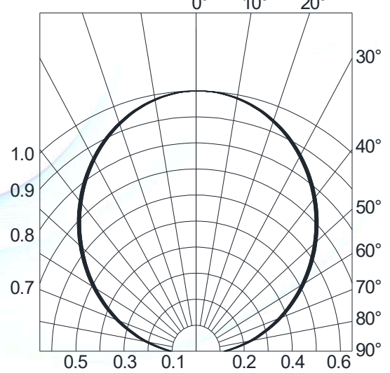
Fig.4-Radiation Diagram T_a=25^{\circ}\text{C}
