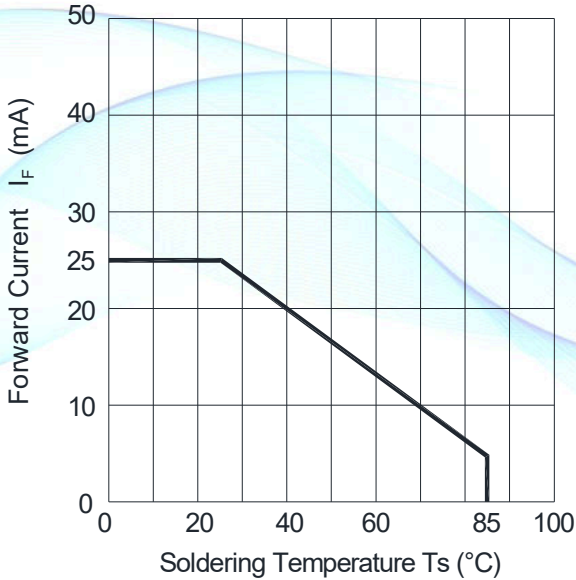
Fig.3-Max. Driving Forward Current vs. Soldering Temperature
