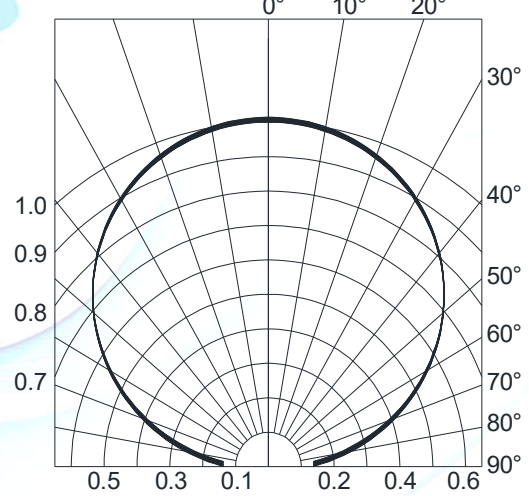
Fig.4-Radiation Diagram T_a=25^{\circ}\text{C}
