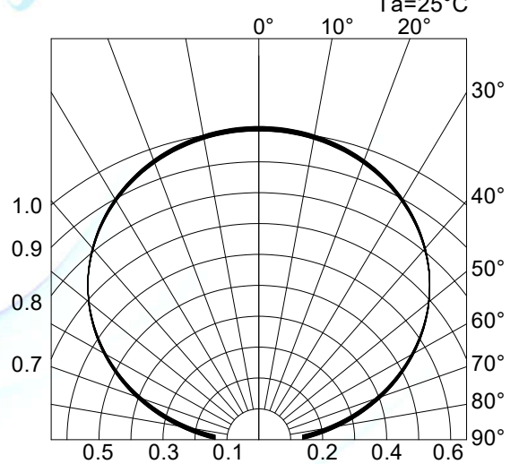
Fig.4-Radiation Diagram T_a=25^\circ\text{C}
