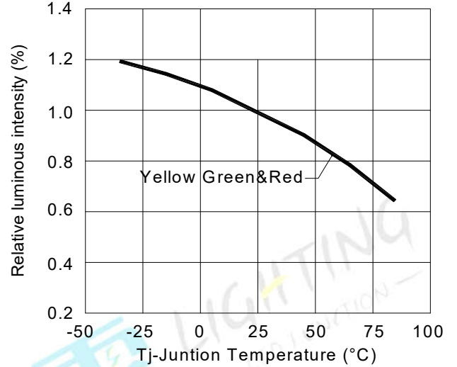
Fig.6-Relative Luminous Intensity vs. Junction Temperature
