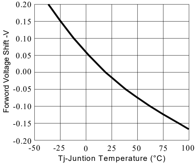
Fig.5-Forward Voltage Shift vs. Junction Temperature
