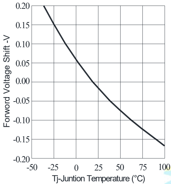
Fig.5-Forward Voltage Shift vs. Junction Temperature
