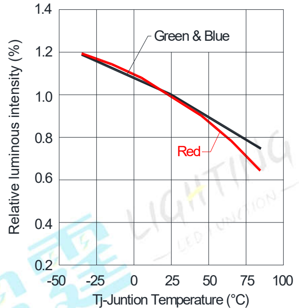
Fig.6-Relative Luminous Intensity vs. Junction Temperature
