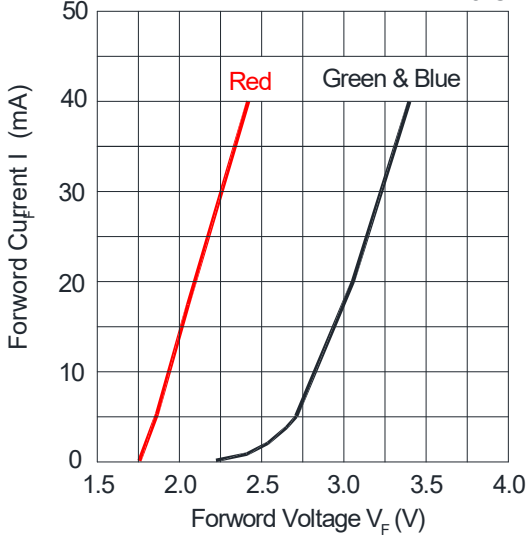
Fig.1-Forward Current(I) vs. Forward Voltage T_s=25^\circ\text{C}
