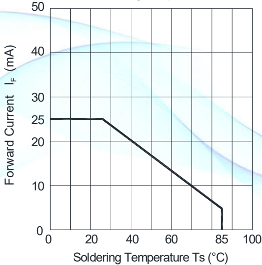
Fig.3-Max. Driving Forward Current vs. Soldering Temperature
