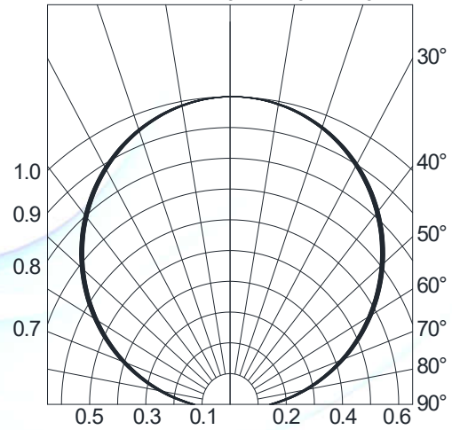
Fig.4-Radiation Diagram T_a=25^\circ\text{C}
