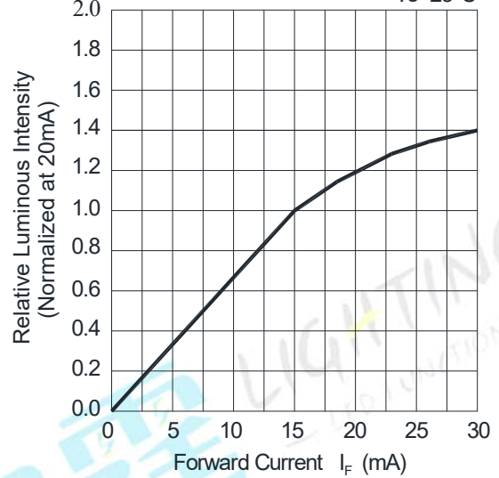
Fig.2-Relative Luminous Intensity vs. Forward Current T_s=25^\circ\text{C}
