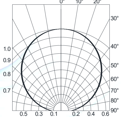
Fig.4-Radiation Diagram T_a=25^\circ\text{C}
