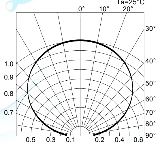
Fig.4-Radiation Diagram T_a=25^\circ\text{C}
