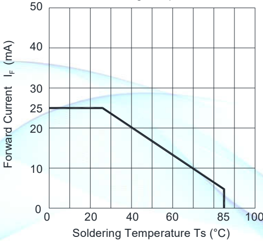
Fig.3-Max. Driving Forward Current vs. Soldering Temperature
