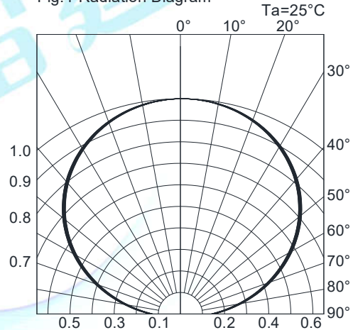
Fig.4-Radiation Diagram T_a=25^\circ\text{C}
