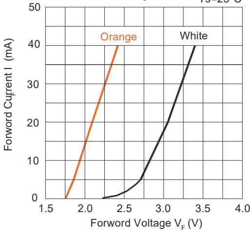
Fig.1-Forward Current(I) vs. Forward Voltage T_s=25^\circ\text{C}
