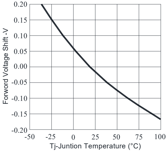
Fig.5-Forward Voltage Shift vs. Junction Temperature
