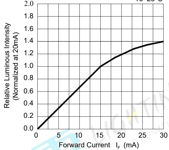
Fig.2-Relative Luminous Intensity vs. Forward Current T_s=25^\circ\text{C}
