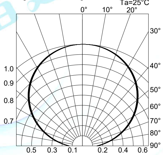
Fig.4-Radiation Diagram T_a=25^\circ\text{C}
