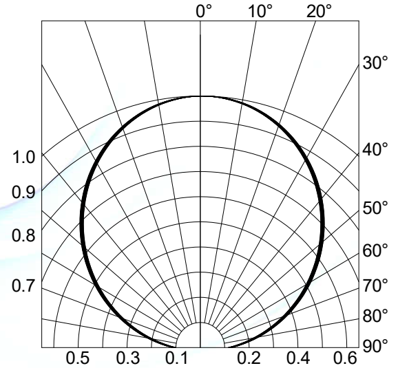
Fig.4-Radiation Diagram T_a=25^{\circ}\text{C}
