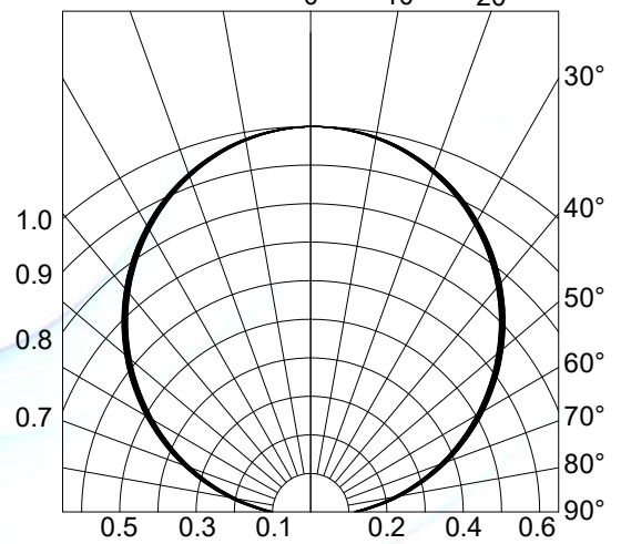
Fig.4-Radiation Diagram T_a=25^\circ\text{C}
